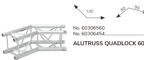
No. 60306555 No. 60306452 .....black ALUTRUSS QUADLOCK 6082C-22 2-Way Corner 120°
